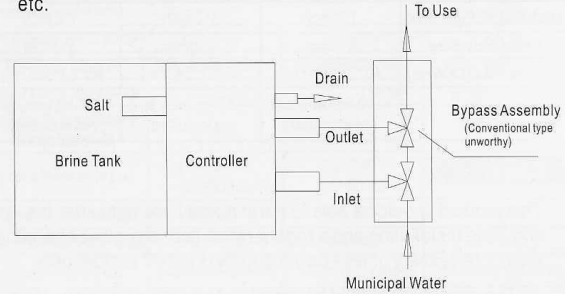
Bypass Assembly Installation Schematic Figure
